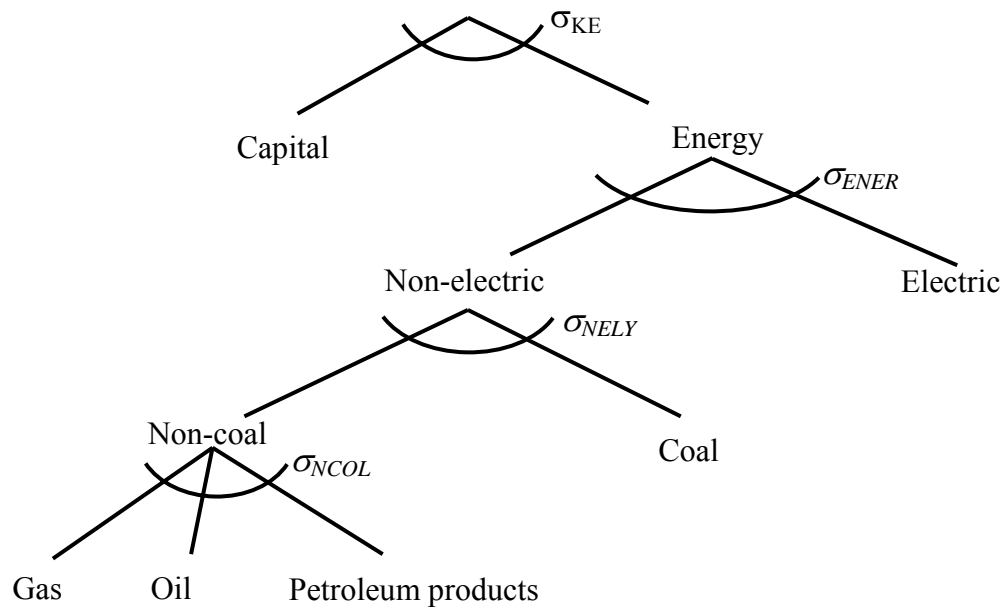
Figure 3: Capital-energy composite in GTAP-E
